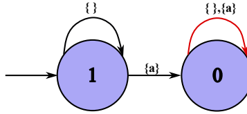
Fig. 1. NBA representing the negated specification \mathbf{F}a . Accepting transitions (highlighted in red) are depicted as self-loops at state q_0 .
